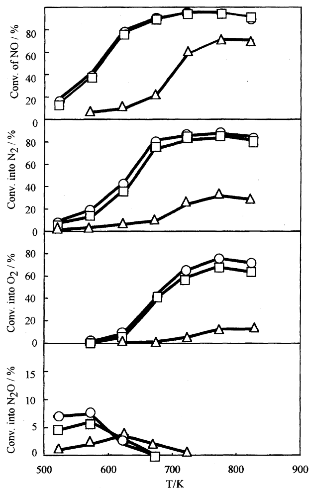
Fig. 3. Temperature dependences of the conversions of NO and into N 2 , O 2 , and N 2 O for NO decomposition catalyzed by Cu/Z-142. ○, W/F=4.0 g s cm -3 ; □, W/F=2.0 g s cm -3 ; △, W/F=0.12 g s cm -3 .
