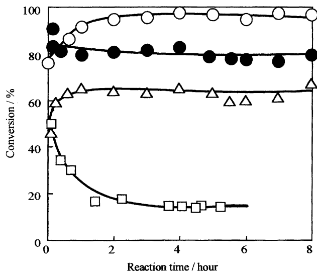
Fig. 2. Time courses of NO and N 2 O decomposition catalyzed by Cu/Z-142. ○, NO; ●, NO into N 2 ; △, NO into O 2 ; W/F=4.0 g s cm -3 ; T=723 K; □, N 2 O into N 2 ; W/F=0.01 g s cm -3 ; T=623 K.
